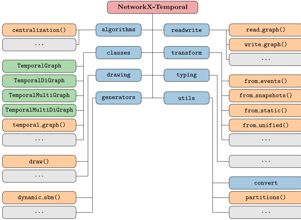
Fig. 1. Overview of software structure. The diagram depicts modules (blue), classes (green), and functions (orange). For brevity, only some classes and functions exposed on package import are shown as examples. Full documentation available online.
