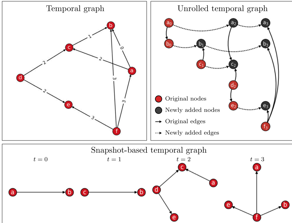
Fig. 2. Temporal graph representations. A directed graph with 6 nodes and 8 edges is represented in static (top left), unrolled (top right), and snapshot-based (bottom) forms. Edges are annotated with a timestamp representing the pairwise interaction time. In the unrolled representation, additional edge couplings linking time-adjacent node copies in the graph are highlighted. All graphs were created and rendered using the software .
