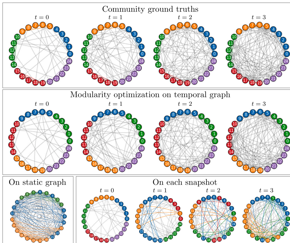
Fig. 3. Community detection on a temporal graph. Graphs were generated by SBM with decreasing assortativeness. We display the node ground truths (top) and the resulting communities obtained by modularity optimization on the unrolled temporal graph (middle), on the static graph (bottom left), and on each snapshot (bottom right). Within-community edges are shown colored. All graphs were rendered using the software. The code to reproduce this example is included in the online software documentation .
