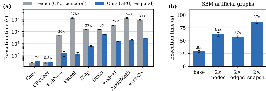
Fig. 2. Runtime evaluation. (a) Execution time of our GPU temporal method against the CPU-bound baseline across real-world datasets (log scale). (b) Effect of independently doubling each axis (nodes, edges, snapshots) on runtime over synthetic SBM instances. Algorithm runs were limited to two iterations only ( leidenalg default). Results reported over five runs; error bars show standard deviation. Experiments conducted on an Intel Xeon Gold 6330 (CPU) and an NVIDIA A100 80GB (GPU).
