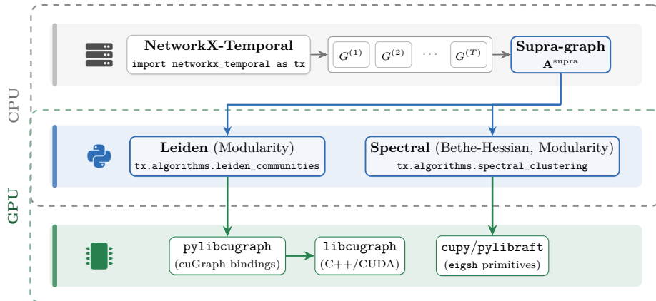
Fig. 1. NetworkX-Temporal integration with cuGraph. Temporal graph snapshots G^{(t)} are assembled into a supra-graph and dispatched through one of two GPU-accelerated paths: multislice modularity via Leiden, or spectral clustering of a (temporal) symmetric modularity or Bethe-Hessian matrix. All methods execute on the RAPIDS ecosystem and return per-snapshot community assignments, allowing zero-code-change execution by setting an environmental variable. In blue: our contributions.
